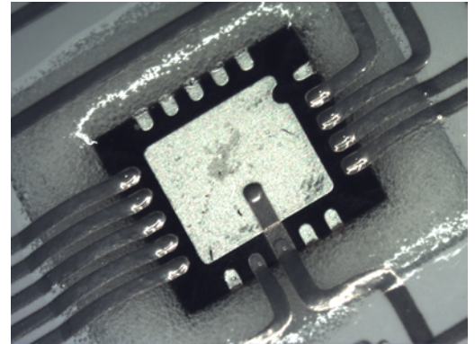
Embedded Electronics
